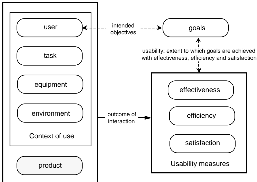
Figure 1 Usability framework
